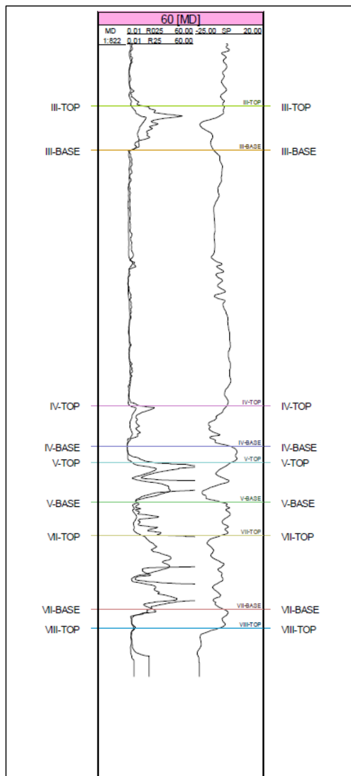
Figure 7: Diagram of the Productive Reservoirs and Log Markers of the Marleysu East Yzbaskent Oilfield
